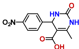
1,2,3,4-Tetrahydro-6-methyl-4-(4-nitrophenyl)- 2-oxo-5-pyrimidinecarboxylic acid
